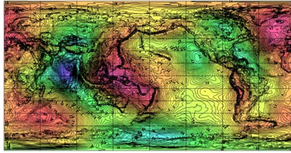
Figure 14 : EGM96 geoid
