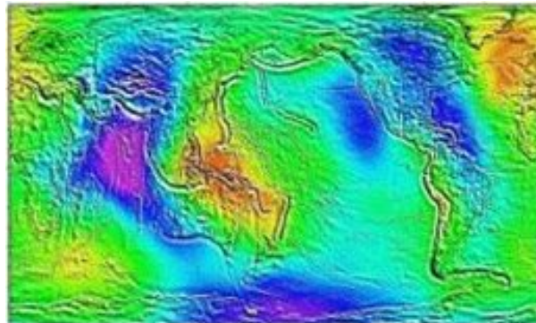
Figure 12 : CLS01 MSS
